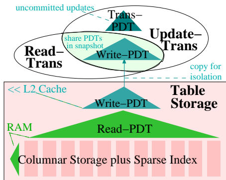
Figure 14: Snapshot Isolation with Layered PDTs
