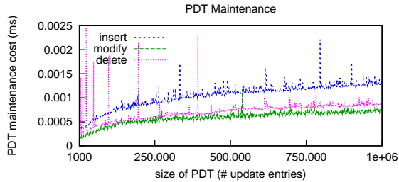
Figure 16: PDT Update Performance Over Time
