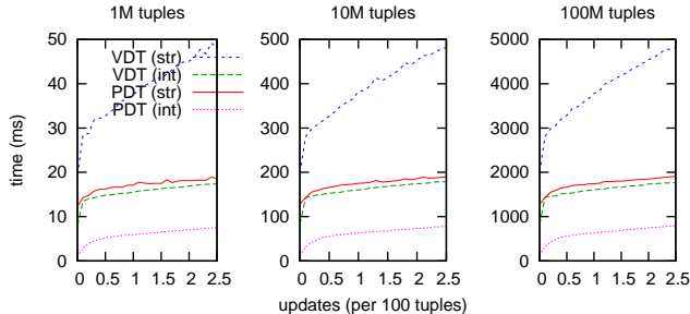
Figure 17: MergeScan: Scaling and Key Type
