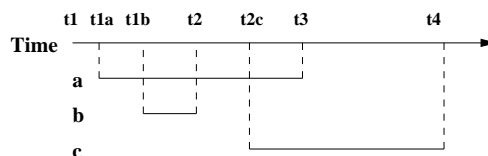
Figure 15: Three Concurrent Transactions
